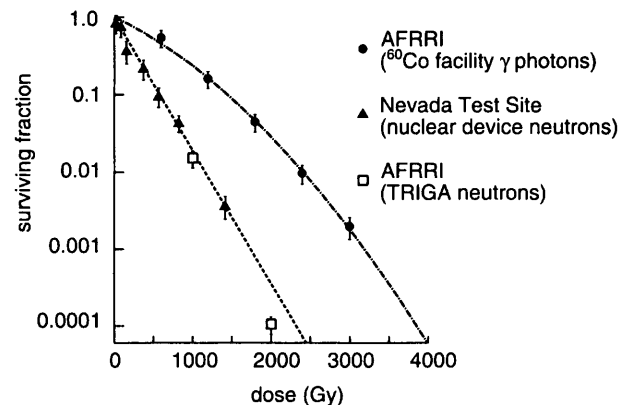
Fig. 1. Spore inactivation by radiation.
