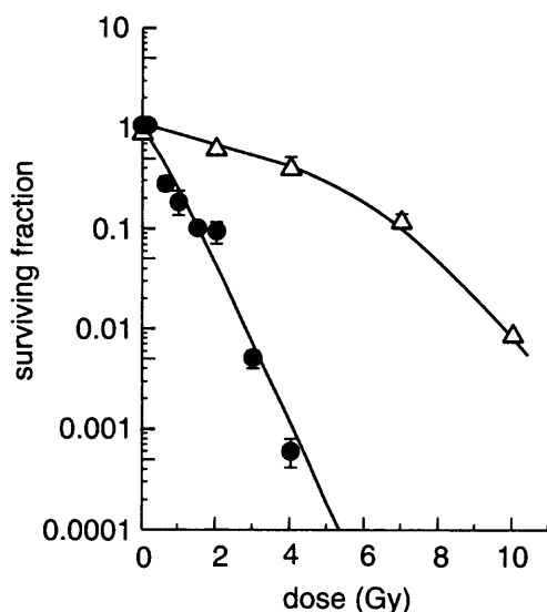
Fig. 3. Clonal survival versus radiation dose response curves. Human CGL1 hybrid cells exposed to cesium 137 \gamma rays ( \Delta ) and AFRRRI fission neutrons ( \bullet ). The cells exposed to \gamma rays were allowed 6 hours of postirradiation incubation before being replated for survival measurements (Redpath et al., 1987). The cells exposed to neutrons were replated for survival measurements immediately after radiation exposure.
